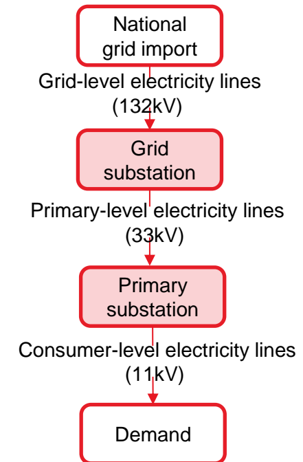
Figure 4.1.8: Modelled electricity flow for each zone
