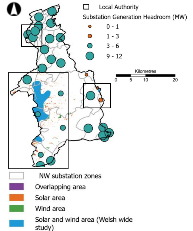
Figure 5.1.12: Areas suitable for wind and ground-mounted solar PV development in Denbighshire and substation generation headroom (MW)
