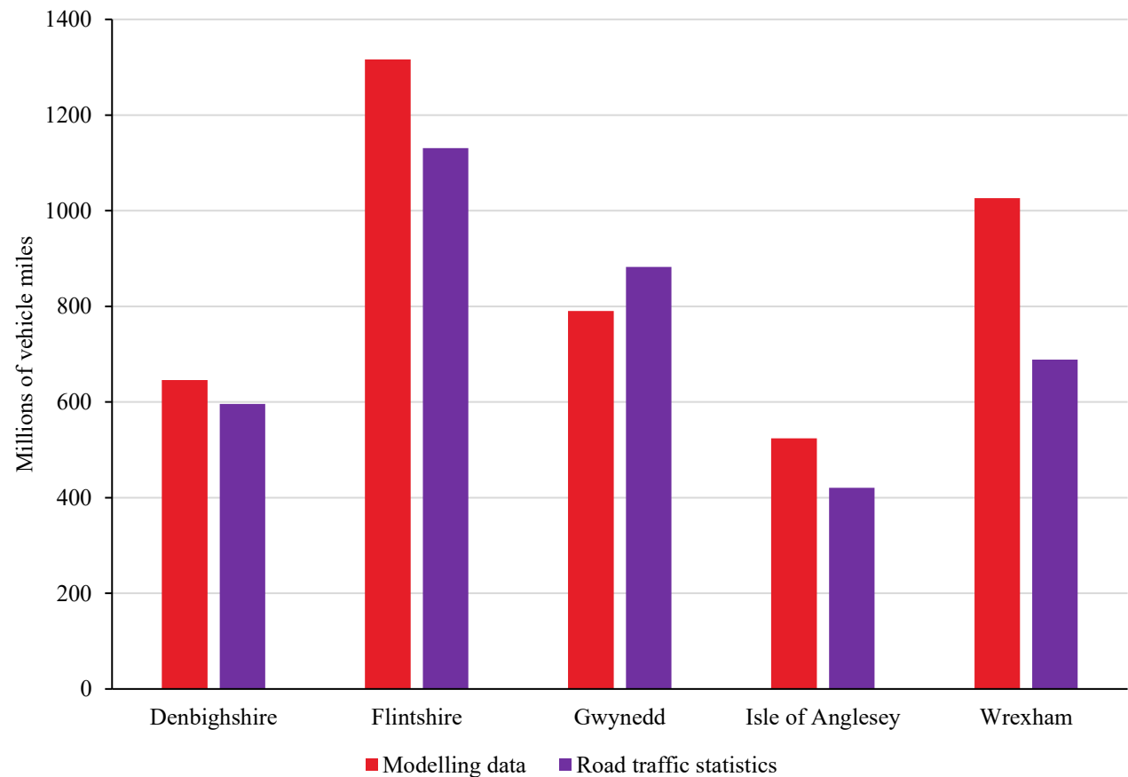
Figure 3.1.5: Comparison of modelling data to DfT road traffic statistics T13
